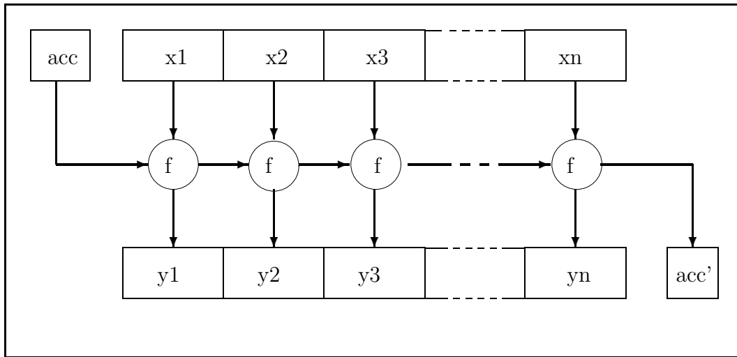
Figure 2.1: A picture of mapAccuml f acc [x 1 , ..., x n ]
