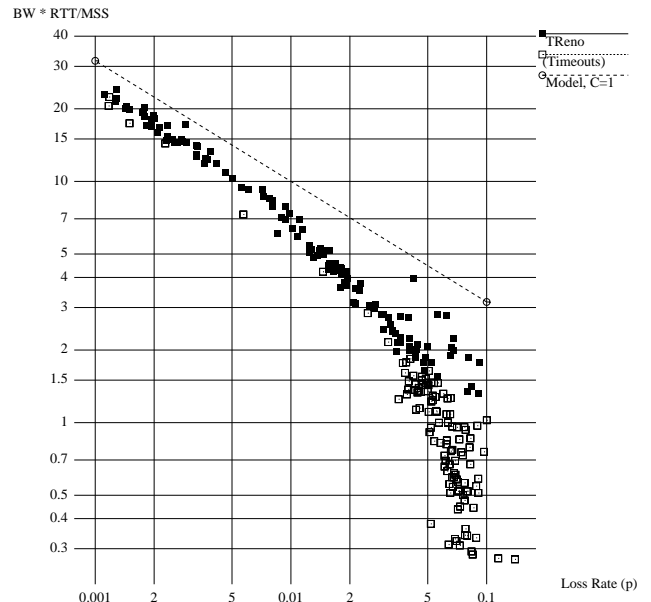
Figure 9: TReno measurement data This data fits Equation 3 with C = 0.744 \pm 0.193 or to Equation 5 with k = -0.617, C = 0.375 \pm 0.054 . These are poorer than the fits in Table 4, in part because the TReno data extends to much worse loss rates, where the effects of rounding become more pronounced. The C values are lower, indicating about 20% lower performance than TCP in a simulator.
