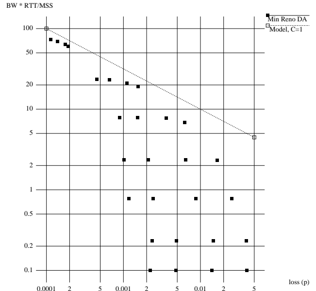
Figure 5: Estimated Window vs. Loss. Simulations of Reno over a bottlenecked link with a drop-tail queue, without correcting for queuing delay. The RTT was 60 ms and the MSS was 1 kbyte. The bandwidth was varied from 10 kb/s to 10 Mb/s, and the queue size was varied from 5 to 30 packets.
