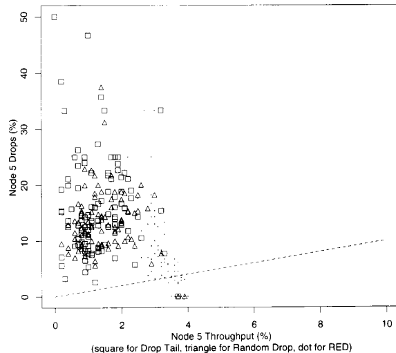
Fig. 15. Scatter plot, packet drops versus throughput.
