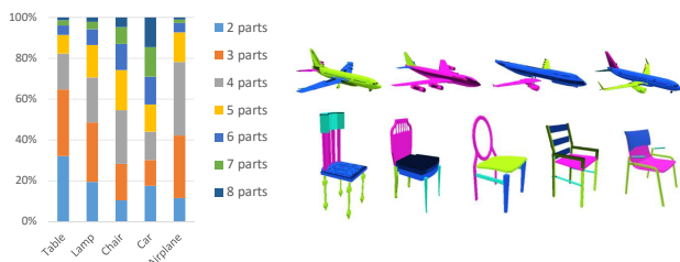
Figure 5. High degrees of inconsistencies exist in the shape segmentations available in the ComplementMe dataset [25]. The left figure charts the distribution of part counts in each object category, showing their diversity. The right figure shows several shapes, within the same category and having the same part counts (3 parts for airplanes, 4 parts for chairs), that exhibit much structural and geometric variation in their segmentations.
