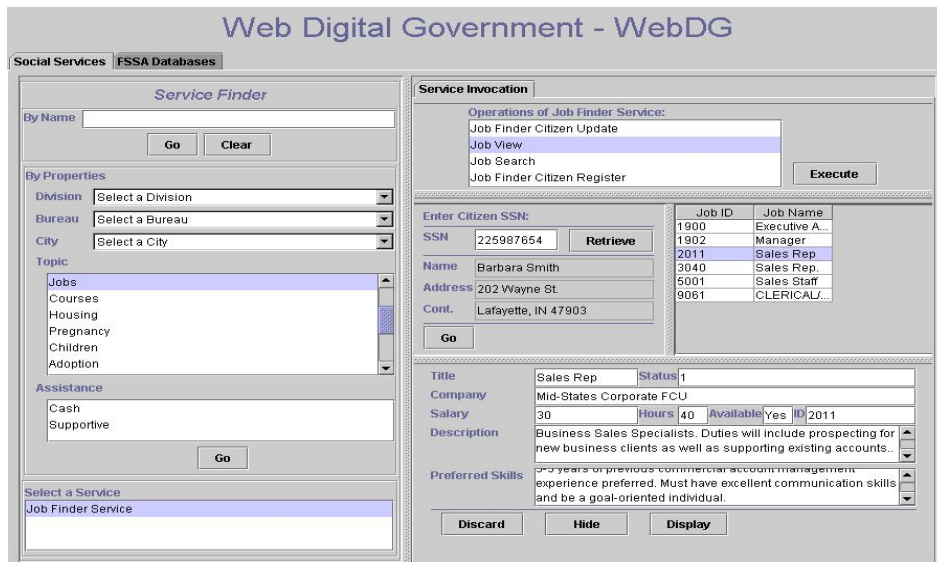
Figure 3: WebDG Interface
