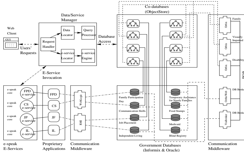
Figure 2: WebDG Architecture
