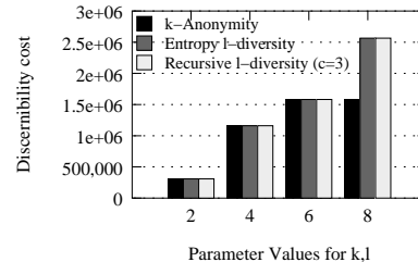
Figure 7. Adults Database. Q = \{\text{age, gender, race, marital\_status}\}
