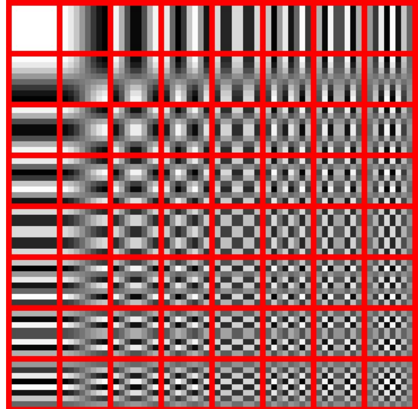
DCT bases
