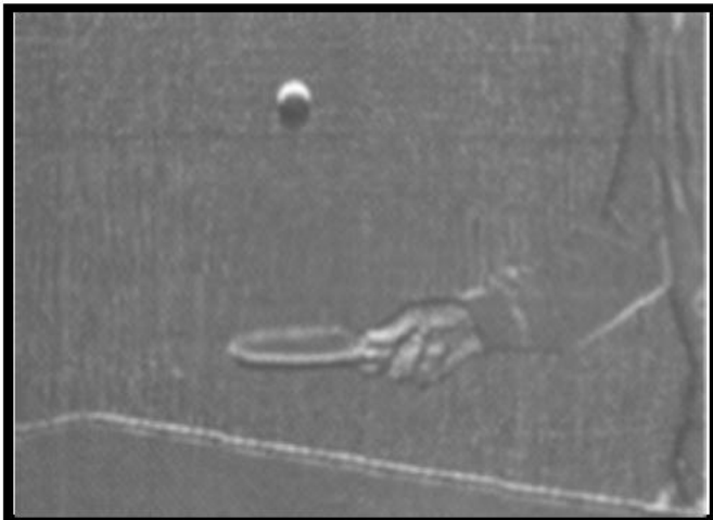
Frame N
