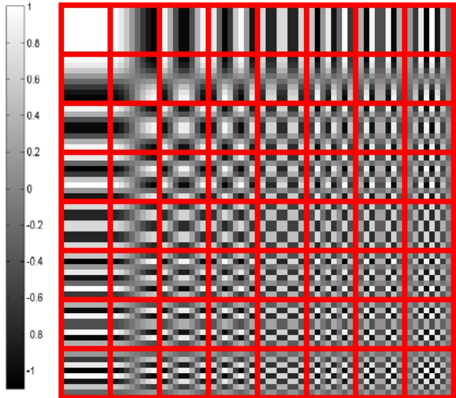
DCT
