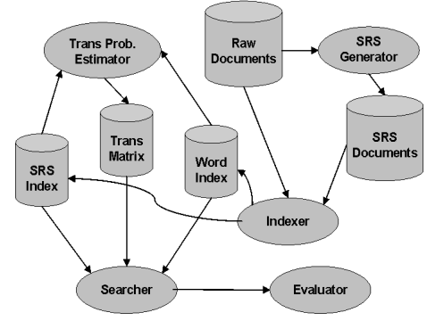
Figure 1: High Level System Architecture
