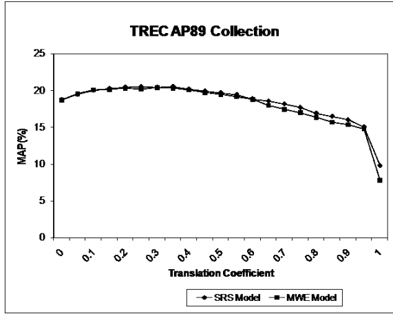
Figure 2: Comparison of the SRS Model with the MWE Topic Signature Model at different values of translation coefficient \lambda
