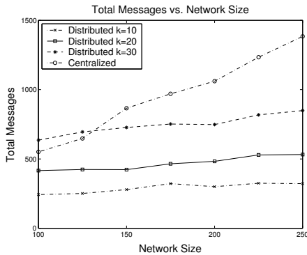
Fig. 5. Messages vs. Nodes
