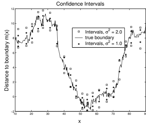
(b) CIs for non-smooth boundary, 100 - \epsilon = 98\%
