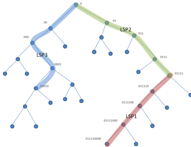
Fig. 3. LSPs in MPLS-TP using OEthernet addressing scheme.
