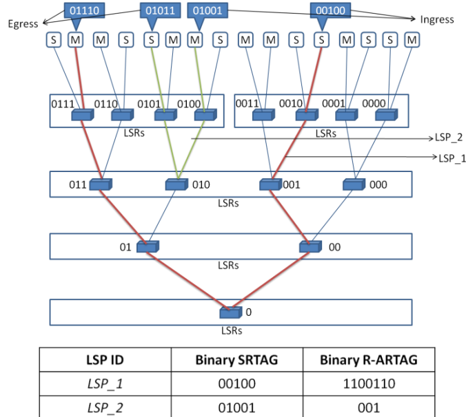
Fig. 7. MPLS-TP data-center and label creation.
