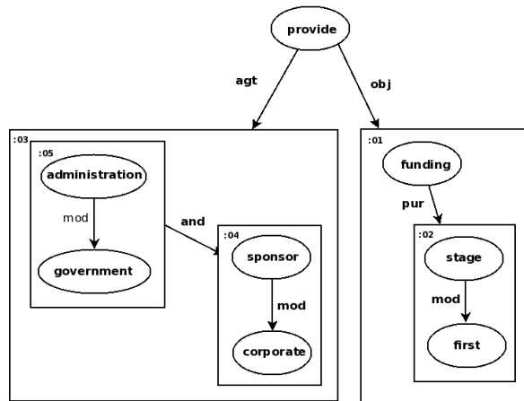
Figure 2: UNL graph for Example 2
