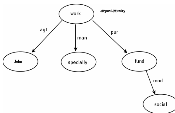
Figure 1: UNL graph for Example 1
