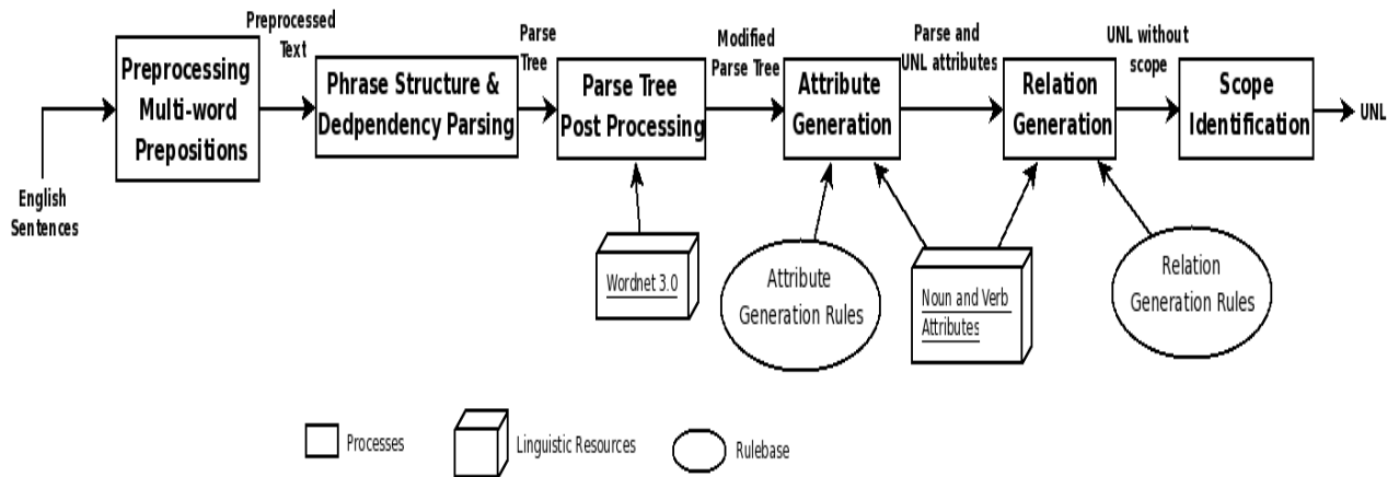
Figure 3 English->UNL Converter Architecture
