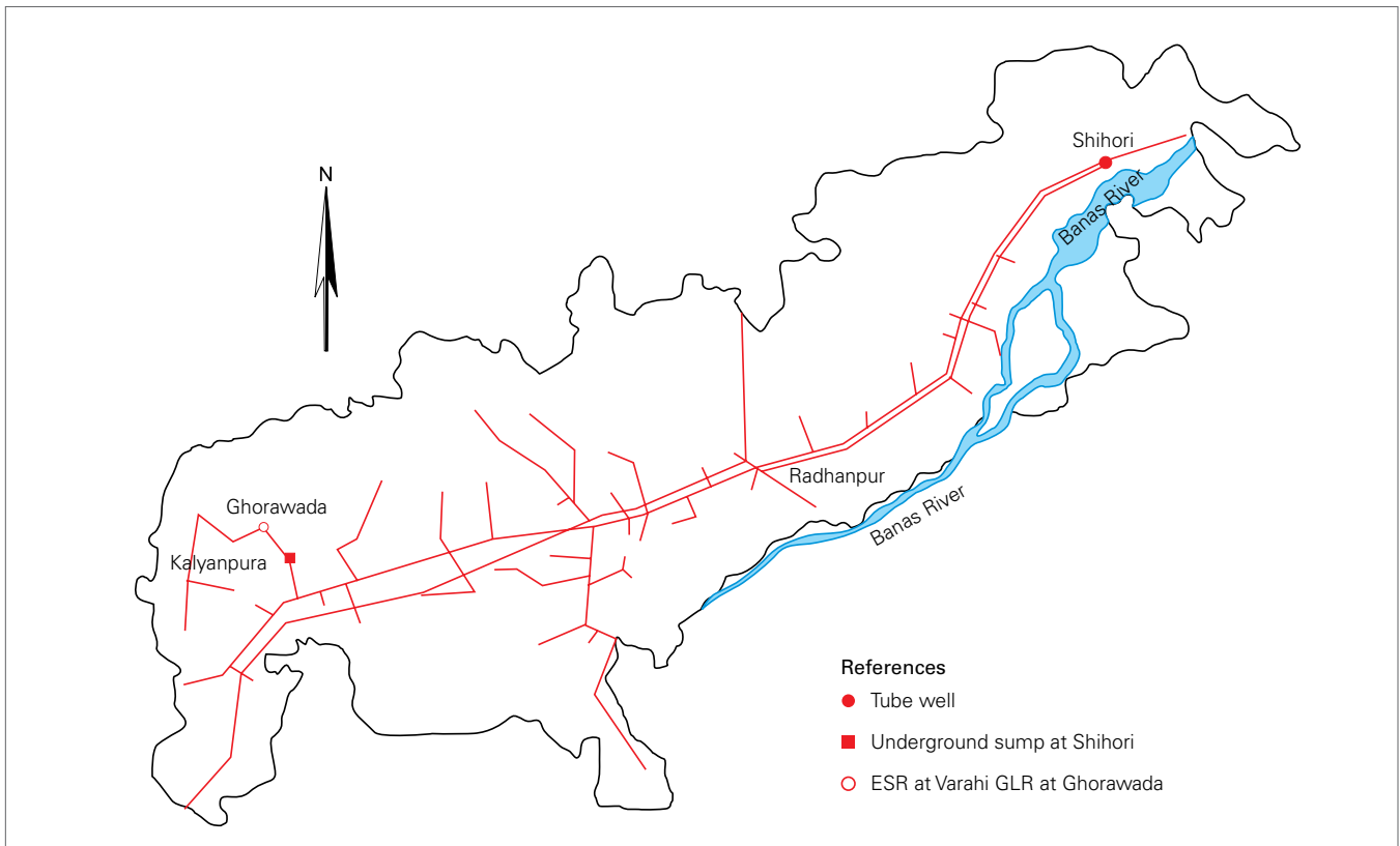
Figure 2.1: Schematic lay out of distribution network of Santalpur regional water supply scheme
