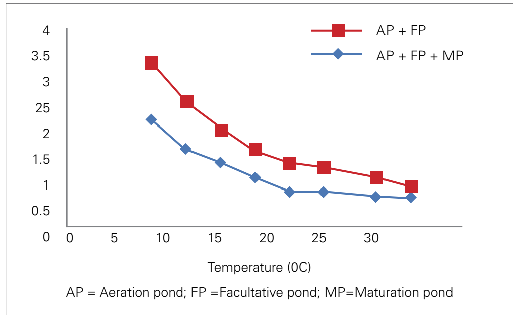
Figure 7.1: Area (m 2 ) required for treatment in WSP at different temperatures
