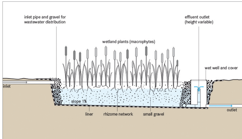
Figure 7.4: Cross-section of subsurface-flow constructed wetland
