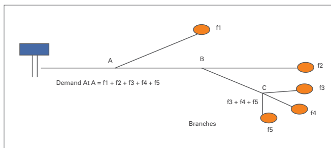
RIGHT: Figure 4A.7: Loop network
