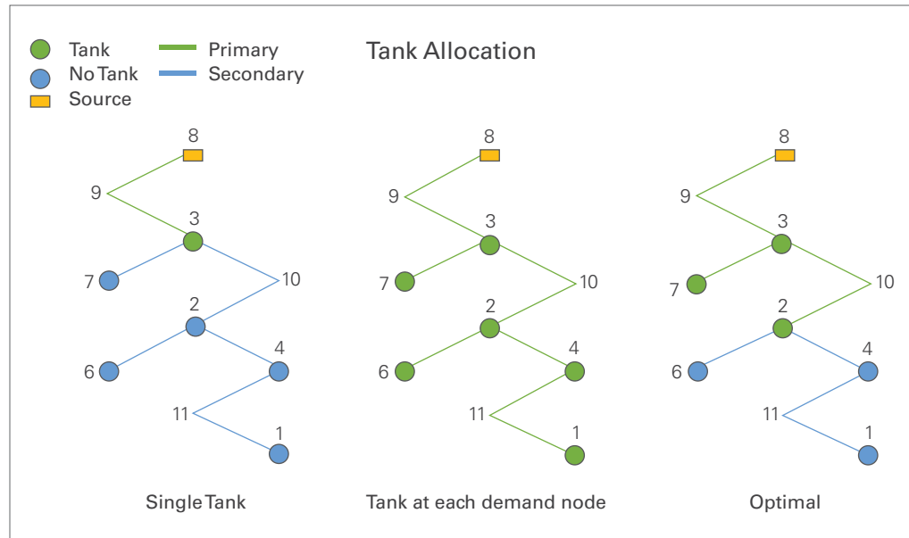
Figure 4C.4: Alternate tank/ESR configurations for a sample network
