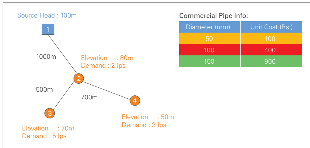
Figure 4C.2: Commercial pipe info
