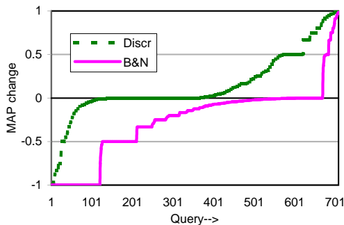
Figure 12: 2-stage entity ranking via B&N does boost accuracy for some queries, but the overall effect is negative. Joint interpretation and ranking also damages some queries but improves many more.
