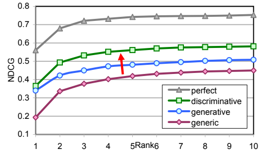
Figure 6: Generic, generative, discriminative and “perfect” accuracies.
