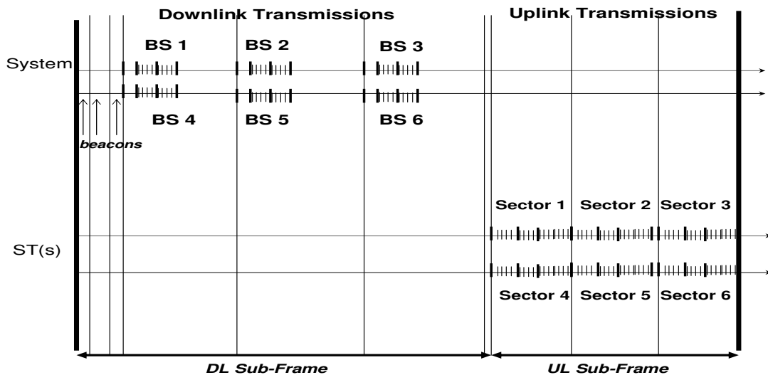
3 4 Figure 8: Parallel transmissions in a six sector system (conservative case)
