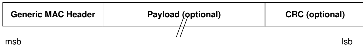
25 Figure 17: MAC PDU format
