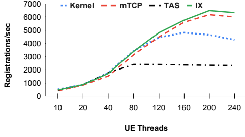
Figure 3: AUSF: Network stack throughput
