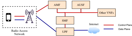
Figure 1: 5G core architecture.
