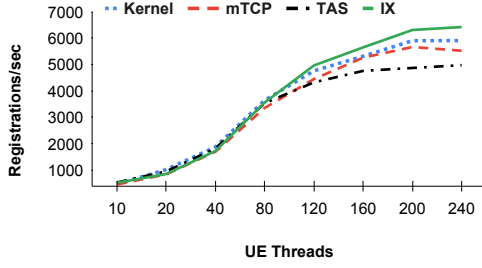
Figure 5: AUSE: Throughput with AMF-Persistent
