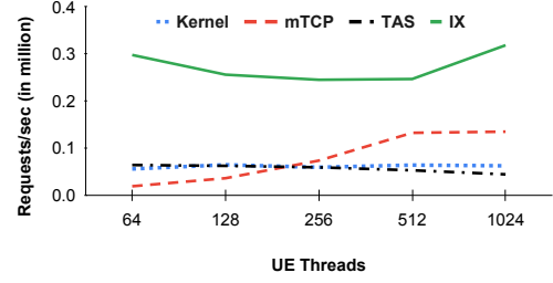
Figure 4: AUSF-IO: Network stack throughput.
