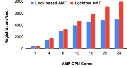
Figure 6: Comparison of lock-based and lock-free AMF
