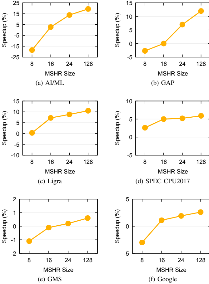
Fig. 3. Performance sensitivity to L1D MSHR size with Berti at L1D, normalized to a 16-entry Standard-MSHR and no L1D prefetcher
