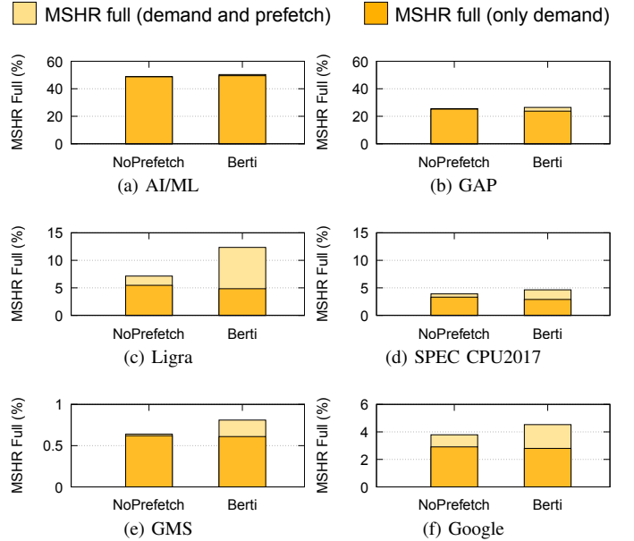
Fig. 2. Percentage of cycles in which all 16 L1D MSHR entries are occupied with no L1D prefetcher and with Berti prefetcher at the L1D. Light bars show total MSHR-full cycles; dark bars show MSHR-full cycles with only demands.
