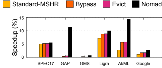
Fig. 7. Ablation of Nomad components with Berti at L1D and 16 L1D MSHR entries
