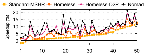
Fig. 13. Multicore speedup with Berti at L1D, normalized to a 16-entry Standard-MSHR without an L1D prefetcher
