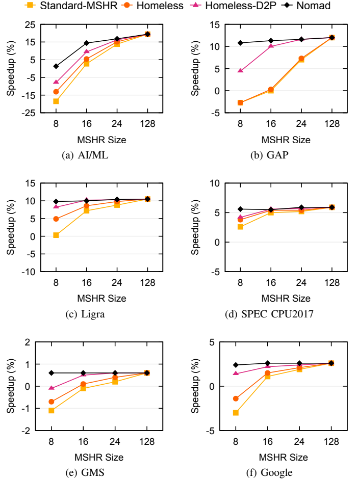
Fig. 5. Performance sensitivity to L1D MSHR size with Berti at L1D, normalized to a 16-entry Standard-MSHR and no L1D prefetcher.
