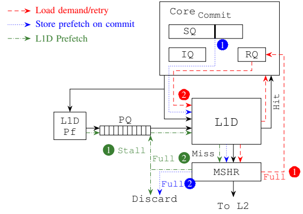
Fig. 1. Overview of actions taken when the MSHR is full
