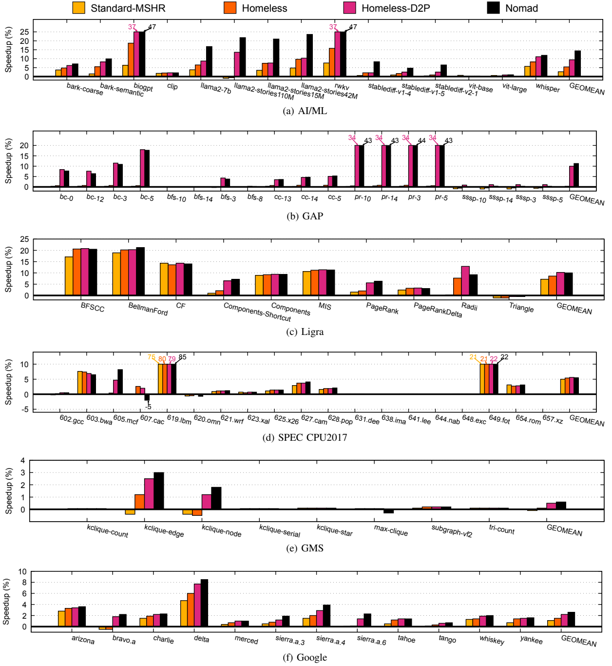
Fig. 6. Per-application speedup with Berti at L1D and a 16-entry L1D MSHR normalized to a 16-entry Standard-MSHR and no L1D prefetcher
