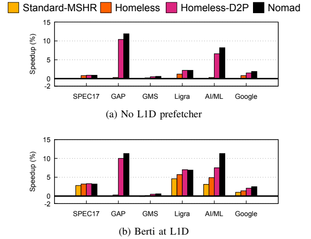
Fig. 8. Performance under limited DRAM bandwidth with 16 L1D MSHR entries
