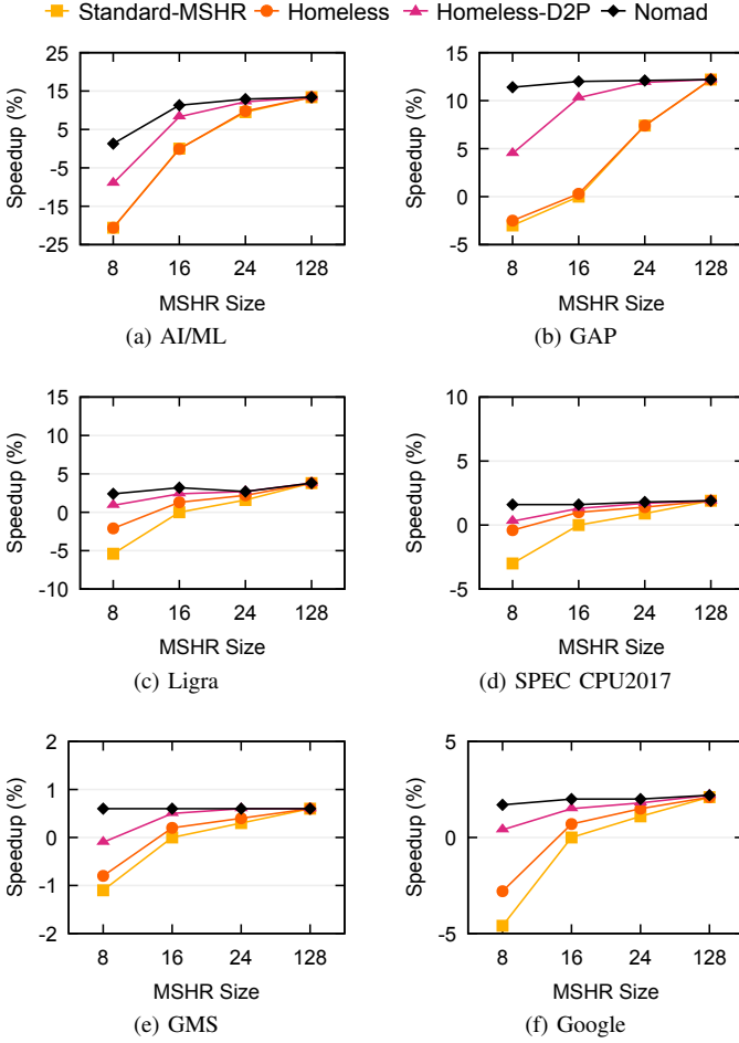
Fig. 4. Performance sensitivity to L1D MSHR size without an L1D hardware prefetcher normalized to a 16-entry Standard-MSHR and no L1D prefetcher
