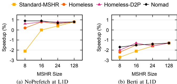
Fig. 14. Sensitivity studies for Splash-4x workloads
