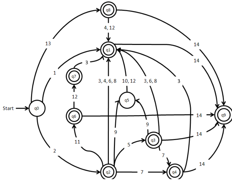
Figure 2. Morphotactic FSM
