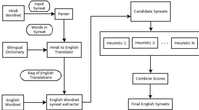
Figure 1: Hindi-English wordnet linking system architecture
