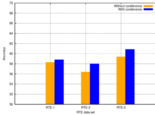
Figure 2: Comparison with coreference and without coreference in the proposed approach
