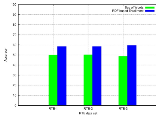
Figure 1: Comparison of Bag of Words and the proposed approach
