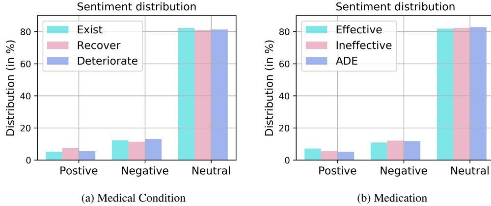
Figure 2: Sentiment word distribution through SentiWordNet
