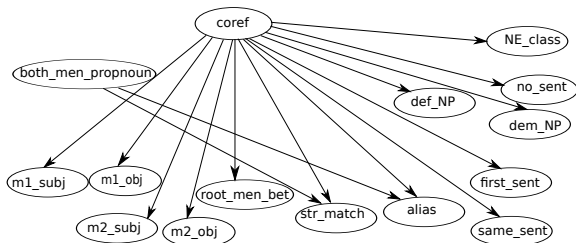
Figure 1: Bayesian network structure depicting dependencies between features
