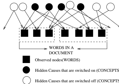
Figure 3: Motivation
