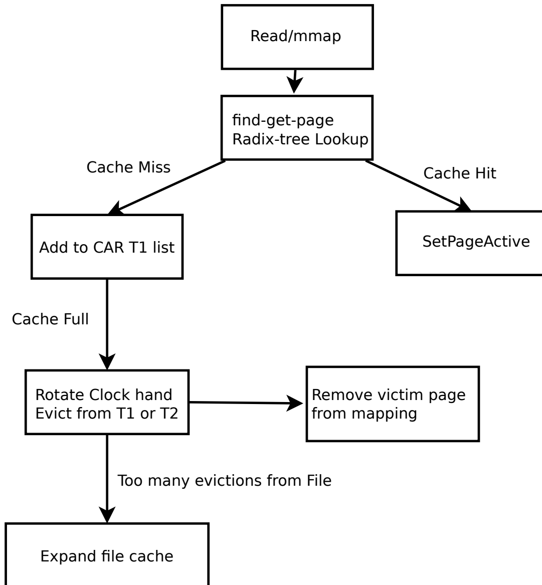
Figure 5.6: Flow-chart of the CAR algorithm implemented. CAR, which acts as the cache-manager for a file, requests the reaper for additional space if it is forced to perform too many evictions
