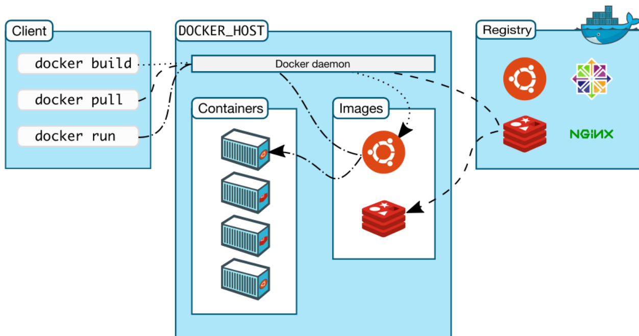
Figure 5.1: Docker Architecture [1]
