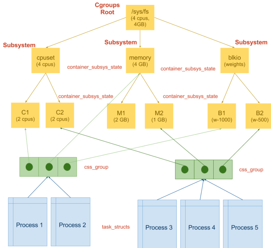
Figure 3.1: simple cgroup illustration using 3 controllers
