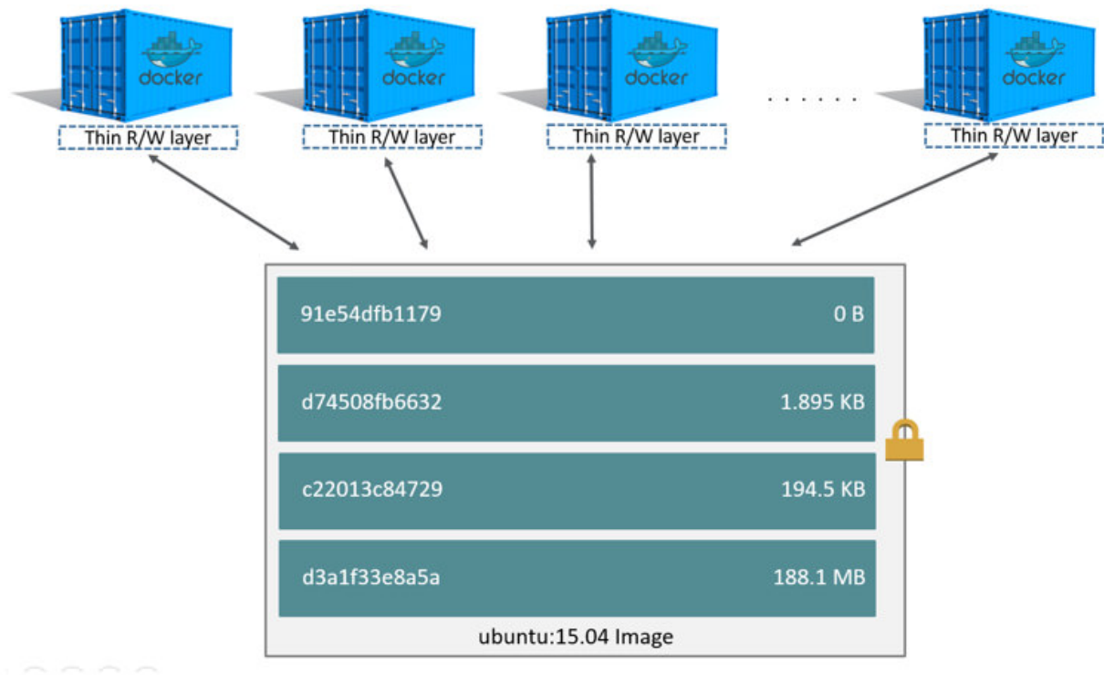
Figure 5.2: Disk layers in Docker [1]
