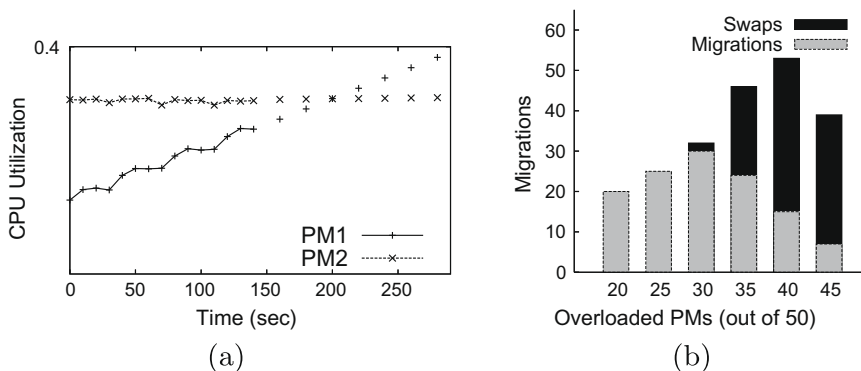
Fig. 11. (a) Using time-series predictions (the dotted lines) allows Sandpiper to better select migration destinations, improving stability. (b) Higher levels of overload requires more migrations until there is no feasible solution.
