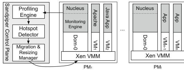
Fig. 1. The Sandpiper architecture.
