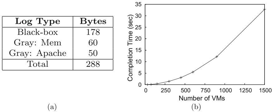
Fig. 10. Sandpiper overhead and scalability.
