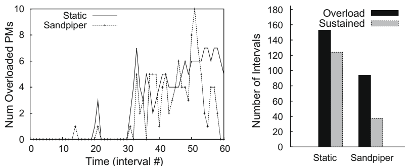
Fig. 9. Sandpiper eliminates all hotspots and reduces the number of intervals experiencing sustained overload by 61%.
