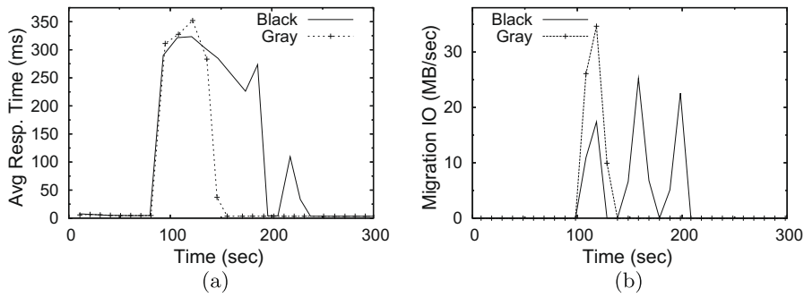
Fig. 8. The gray-box system balances the system more quickly due to more informed decision making. The black-box system must perform migrations sequentially and incurs an additional migration.
