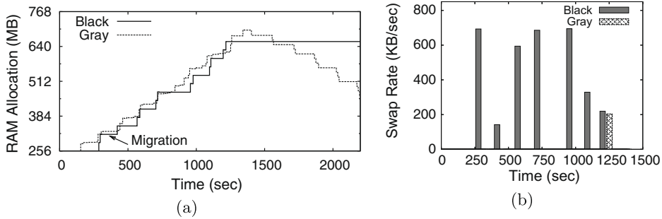
Fig. 6. The black-box system lags behind the gray-box system in allocating memory. The gray-box approach proactively increases memory and safely reduces the VM's memory allocation when demand falls.
