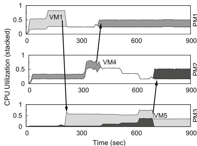
Fig. 4. A series of migrations resolve hotspots. Different shades are used for each migrating VM.
