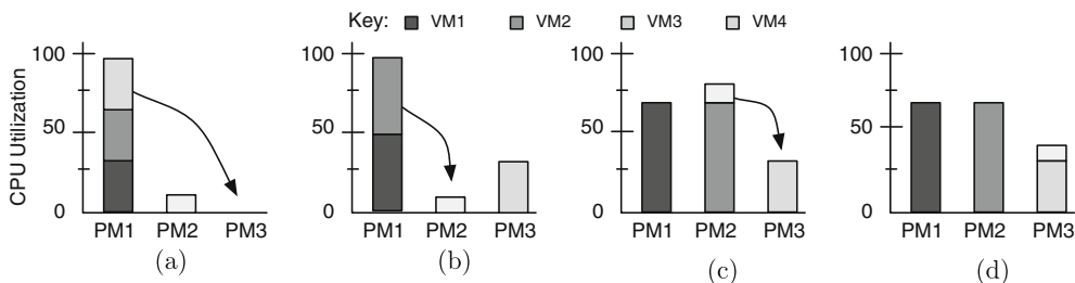
Fig. 7. The black-box system incorrectly guesses resource requirements since CPU usage is saturated, resulting in an increased resolution time. The gray-box system infers usage requirements and transitions directly from (a) to (d).
