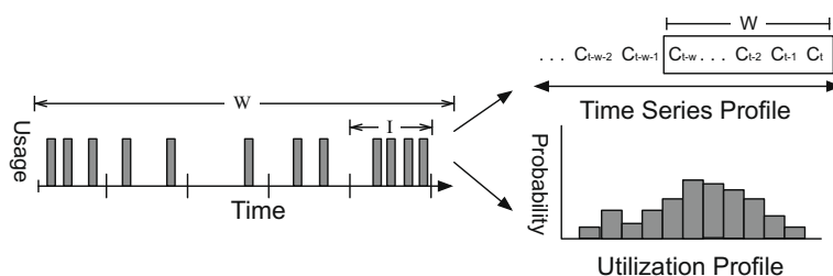
Fig. 2. Profile generation in Sandpiper
