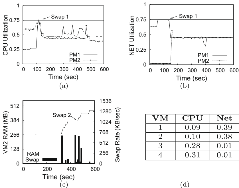
Fig. 5. Swaps and migrations to handle network- and memory-intensive loads. Initially, VM 1 and VM 2 are on PM 1 , the rest on PM 2 . After two swaps, PM 1 hosts VM 1 and VM 4 .
