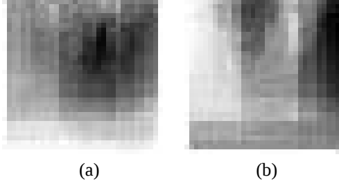
Figure 4.(a) The most and the (b) the second most prominent Eigen Block Directional Fingerprint of a left loop classification template image. The grey values correspond to a scaled encoding of the quantised set of directions in a block.
