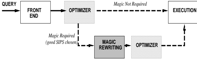
Figure 3: Optimization Architecture
