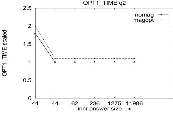
Figure 8: Initial Optimizer Overhead
