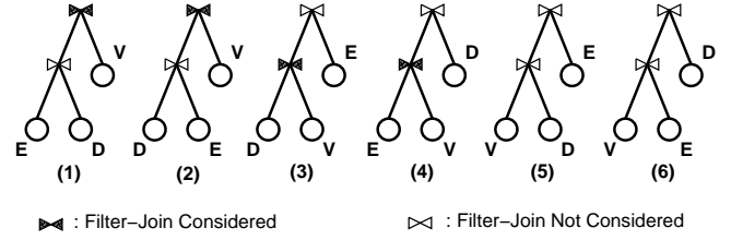
Figure 4: Some Possible Join Orders
