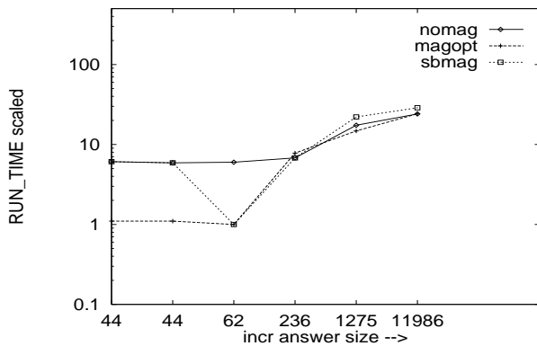
Figure 5: Overall Comparison
