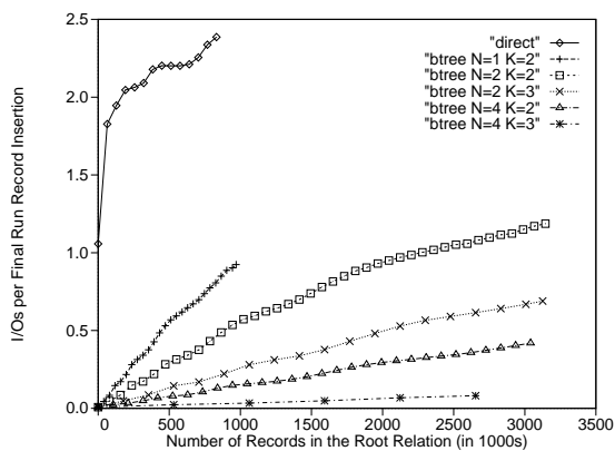
Figure 3: Stepped-Merge: Cost of Insertion into Root Relation
