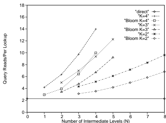
Figure 5: Stepped-Merge: Cost of Lookups
