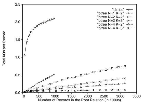
Figure 1: Stepped-Merge: Total Insertion Cost
