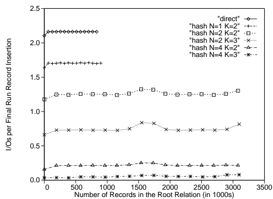
Figure 4: Stepped-Hash: Cost of Insertion into Root Relation
