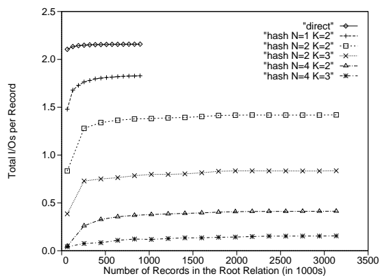
Figure 2: Stepped-Hash: Total Insertion Cost
