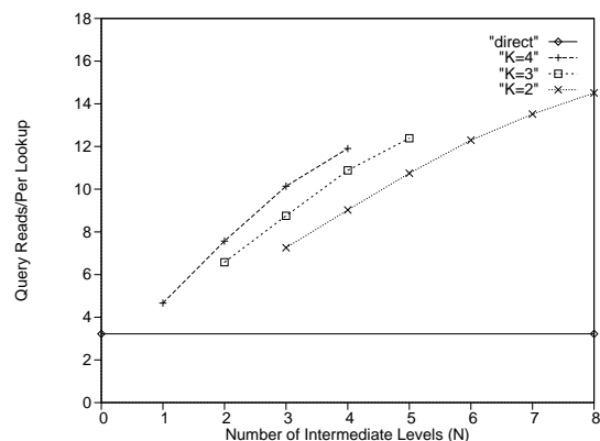
Figure 6: Stepped-Hash: Cost of Lookups
