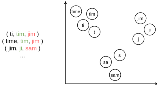
Figure 4: Illustration of Triplet Loss
