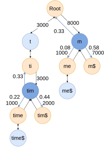
Figure 3: A portion of the suffix Tree from Figure 1 annotated with transition probabilities based on Equation 5.
