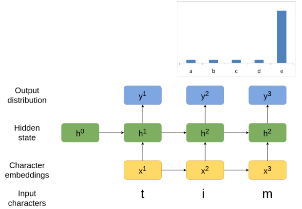
Figure 5: Illustration of a simple Neural Language Model used in ASTRID-NLM. The bar chart provides the probability distribution p(\cdot | BOW, t, i, m) . The character e seems to be most likely one.
