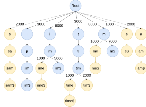
Figure 1: Generalized (uncompressed) Suffix tree for strings \{‘sam’, ‘jim’, ‘tim’, ‘time’\}
