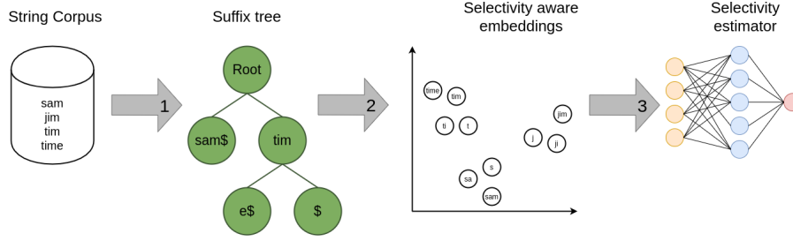
Figure 2: Major components of ASTRID-EMBED
