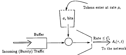
Fig. 3. A Leaky Bucket.
