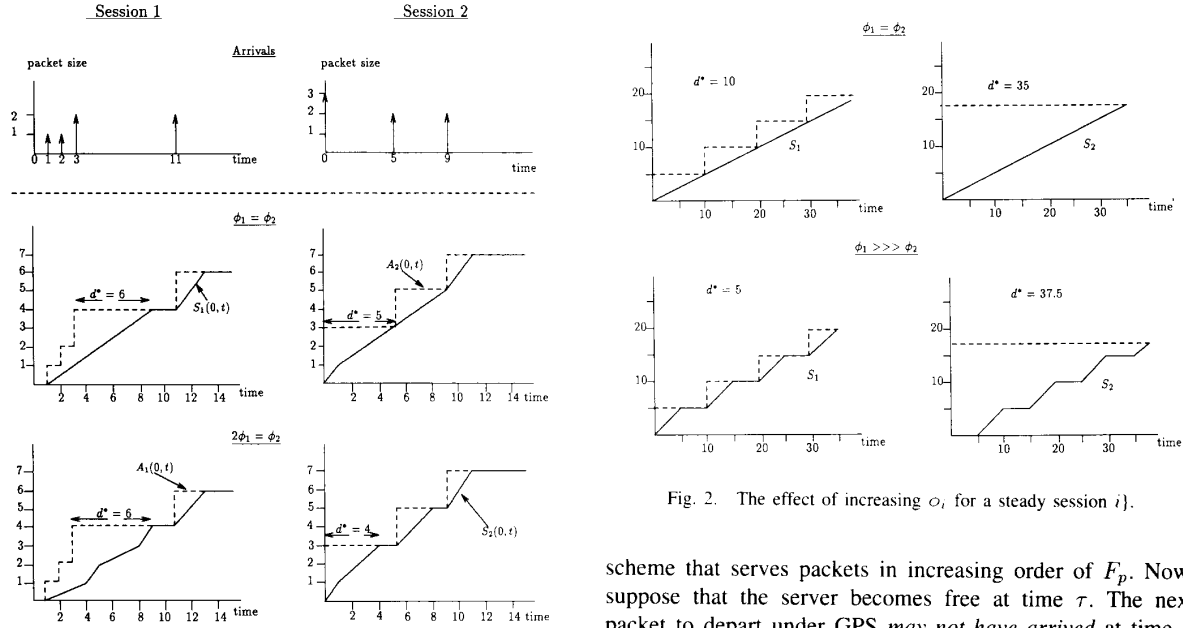
Fig. 1. An example of generalized processor sharing.
