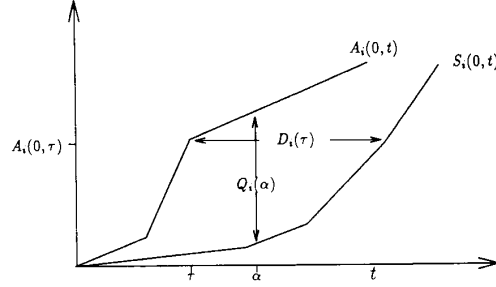
Fig. 5. A_i(0, t) , S_i(0, t) , Q_i(t) and D_i(t)
