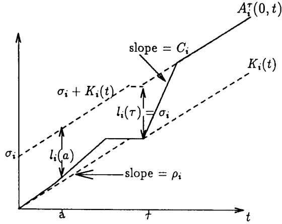
Fig. 6. A session i arrival function that is greedy from time \tau .
