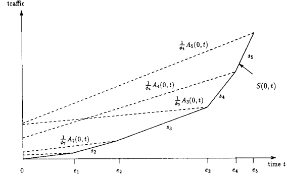
The arrival functions are scaled so that a universal service curve, S(0, t) , can be drawn. After time e_i , session i has a backlog of zero until the end of the system busy period, which is at time e_N . The vertical distance between the dashed curve corresponding to session i and S(0, \tau) is \frac{1}{\phi_i} Q_i(\tau) , while the horizontal distance yields D_i(\tau) just as it does in Figure 8.
