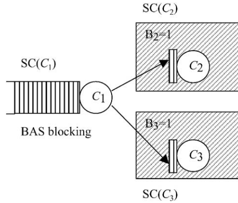
Fig. 5. Modeling one to two synchronous communication between concurrent components.
