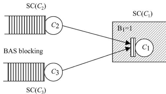
Fig. 6. Modeling two to one synchronous communication between concurrent components.
