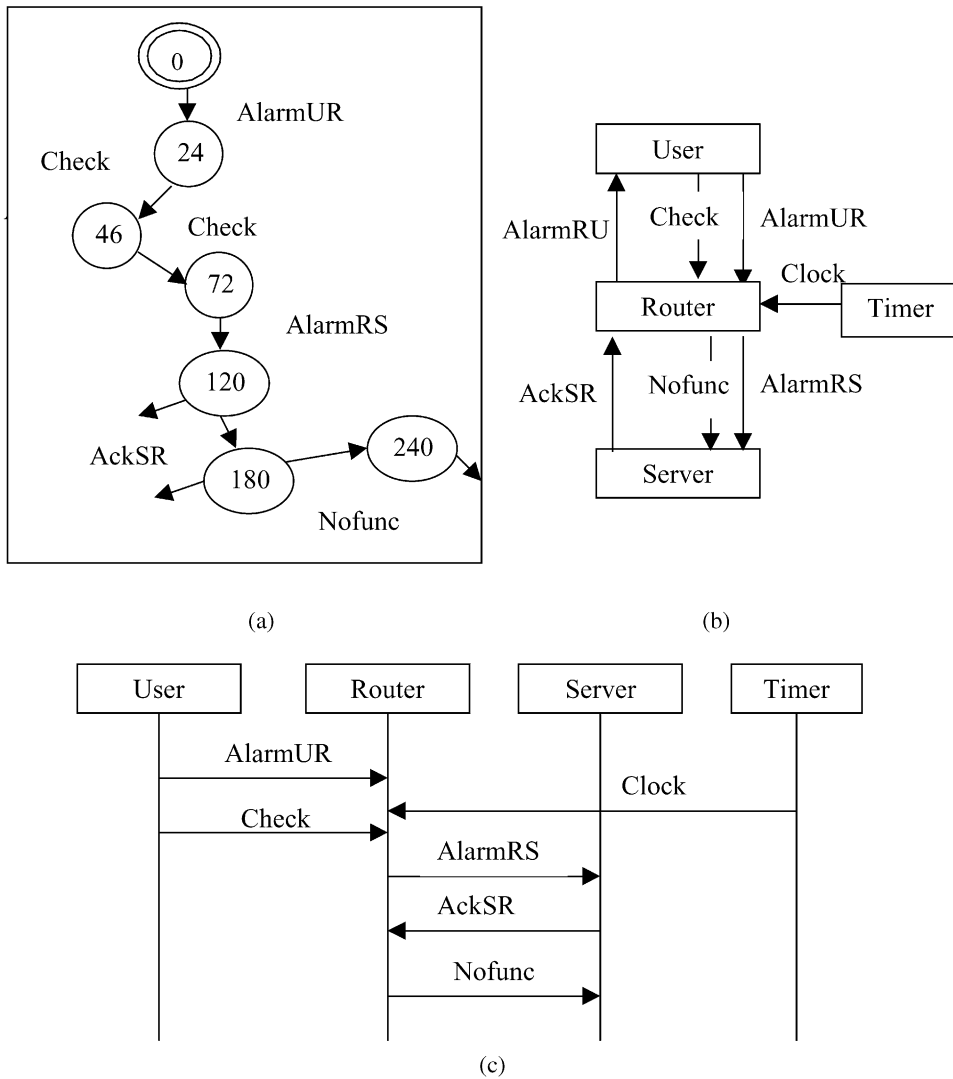
Fig. 2. Dynamic views (a) a portion of the FSM, (b) static view, (c) MSC.
