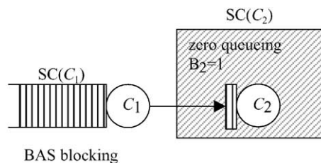
Fig. 4. Modeling synchronous communication between concurrent components.
