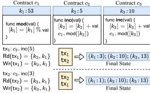
Figure 1: Contract c_1 , c_2 and c_3 with their initial state \{(k_1 : 53), (k_2 : 5) \text{ and } k_3 : 10\} , respectively. Transaction tx_1 and tx_2 are two transactions that update these states according to the specified program logic.
