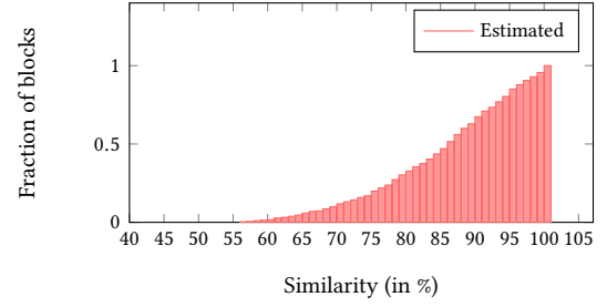
Figure 4: Cumulative average estimated similarity at host nodes running go-ethereum implementation.
