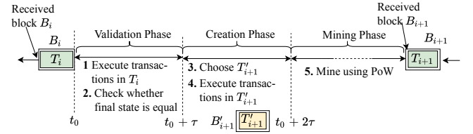
Figure 2: Serialization of the block validation phase, block creation phase and mining phase
