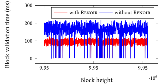
Figure 11: Validation time of 1000 real Ethereum blocks at two nodes, one of which is equipped with RENOIR and the other is not.
