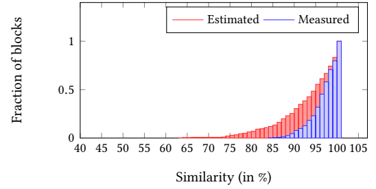
Figure 5: Cumulative similarity at our instrumented go-ethereum nodes \{n_1, \dots, n_{10}\} . The measured similarity reports the actual similarity observed at these nodes and the estimated similarity reports our estimation of similarity at n_1 to n_{10} using a different probe node n_{11} .
