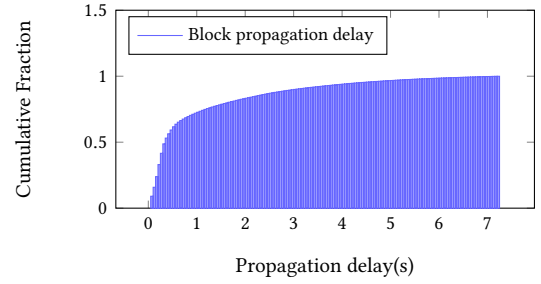
Figure 8: Block propagation delay in Ethereum network.
