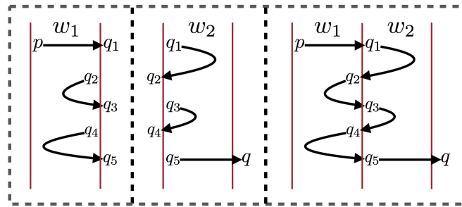
Figure 3 The first and second pictures are illustrations of subsets of \text{Tr}(w_1) and \text{Tr}(w_2) respectively. (p, \rightarrow, q_1), (q_2, \zeta, q_3), (q_4, \zeta, q_5) \in \text{Tr}(w_1) while (q_1, \rhd, q_2), (q_3, \rhd, q_4), (q_5, \rightarrow, q) \in \text{Tr}(w_2) . The third picture shows that (p, \rightarrow, q) \in \text{Tr}(w_1 \cdot w_2) : (p, \rightarrow, q) consists of “steps” (p, \rightarrow, q_1), (q_1, \rhd, q_2), (q_2, \zeta, q_3), (q_3, \rhd, q_4), (q_4, \zeta, q_5), (q_5, \rightarrow, q) alternately from \text{Tr}(w_1) and \text{Tr}(w_2) .
