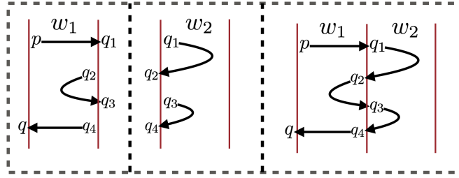
Figure 4 Let w = w_1 \cdot w_2 \in \mathcal{L}(E) with w_1 \in \mathcal{L}(E_1) , w_2 \in \mathcal{L}(E_2) . We have (p, \rightarrow, q_1), (q_2, \prec, q_3), (q_4, \leftarrow, q) \in \text{Tr}(w_1) and (q_1, \succ, q_2), (q_3, \succ, q_4) \in \text{Tr}(w_2) . Then (p, \succ, q) is composed of “steps” (p, \rightarrow, q_1), (q_1, \succ, q_2), (q_2, \prec, q_3), (q_3, \succ, q_4), (q_4, \leftarrow, q) alternately from \text{Tr}(w_1) and \text{Tr}(w_2) .
