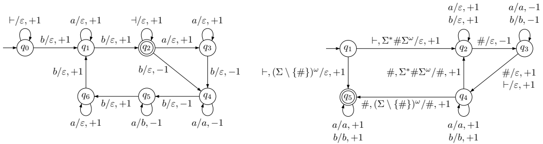
Figure 1 On the left, a 2DFT \mathcal{A} with [[\mathcal{A}]](ba^{m_1}ba^{m_2}b \dots a^{m_k}b) = a^{m_2}b^{m_1}a^{m_3}b^{m_2} \dots a^{m_k}b^{m_{k-1}} . On the right, an \omega -2DMTla \mathcal{A}' with [[\mathcal{A}']](u_1\#u_2\# \dots \#u_n\#v) = u_1^R u_1 \# u_2^R u_2 \# \dots \# u_n^R u_n \# v where u_1, \dots, u_n \in (a+b)^* , v \in (a+b)^\omega and u^R denotes the reverse of u . The Muller acceptance set is \{\{q_5\}\} . The look-ahead expressions \Sigma^* \# \Sigma^\omega and (\Sigma \setminus \{\#\})^\omega are used to check if there is a \# in the remaining suffix of the input word.
