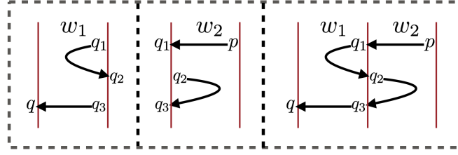
Figure 5 Let w = w_1 \cdot w_2 \in \mathcal{L}(E) with w_1 \in \mathcal{L}(E_1) , w_2 \in \mathcal{L}(E_2) . We have (p, \leftarrow, q_1), (q_2, \rhd, q_3) \in \text{Tr}(w_2) and (q_1, \zeta, q_2), (q_3, \leftarrow, q) \in \text{Tr}(w_1) . Then (p, \leftarrow, q) \in \text{Tr}(w) is composed of “steps” (p, \leftarrow, q_1), (q_1, \zeta, q_2), (q_2, \rhd, q_3), (q_3, \leftarrow, q) alternately from \text{Tr}(w_2) and \text{Tr}(w_1) .
