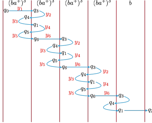
Figure 10 run of a word in E_3 = [(ba^+)^3]^+b
