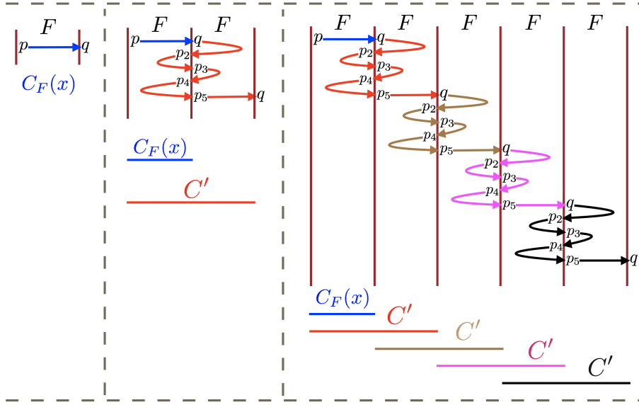
Figure 6 In the Kleene-plus E = F^+ , a step x = (p, \rightarrow, q) \in s_E on some u = u_1 u_2 \cdots u_n with u_\ell \in \mathcal{L}(F) is obtained by composing the following steps in s_F : x_1 = x , x_2 = (q, \rhd, p_2) , x_3 = (p_2, \zeta, p_3) , x_4 = (p_3, \rhd, p_4) , x_5 = (p_4, \zeta, p_5) , x_6 = (p_5, \rightarrow, q) .
