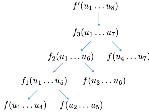
Figure 12 Computation of f'(u_1 \cdots u_8)
